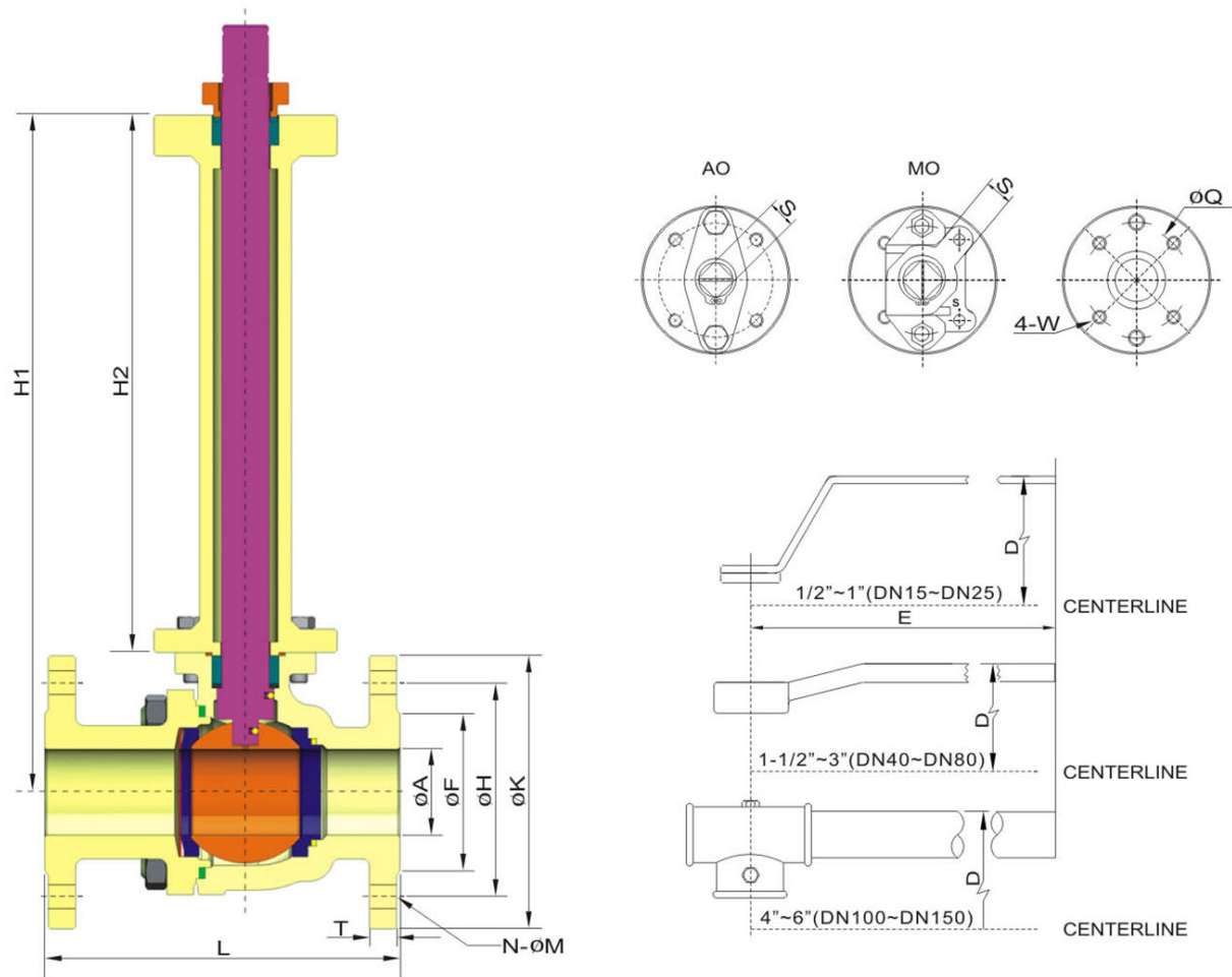
DIMENSIONS (JBF/JBFM-A1 SERIES JIS 10K)
