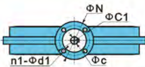
Size DN700 to DN1200
