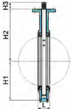
Size DN25 to DN600
