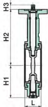
Size DN40 to DN300
