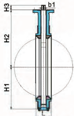
Size DN700 to DN800
