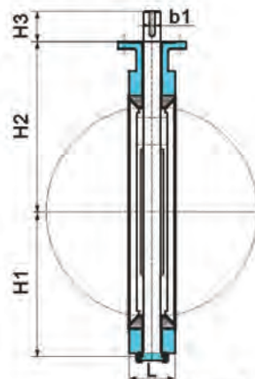
Size DN700 to DN1200
