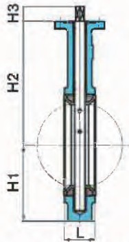
Size DN25 to DN600
