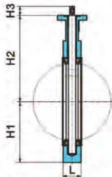
Size DN40 to DN600
