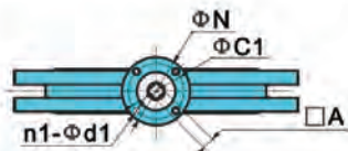
Size DN40 to DN600
