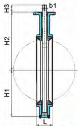
Size DN700 to DN1200
