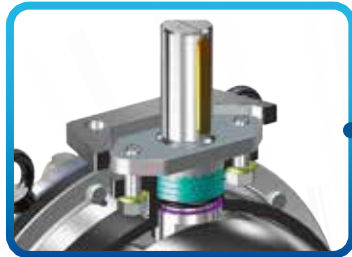
Adjustable Gland
