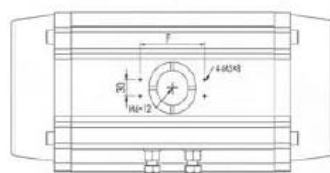
JEW/JEV-210-350
